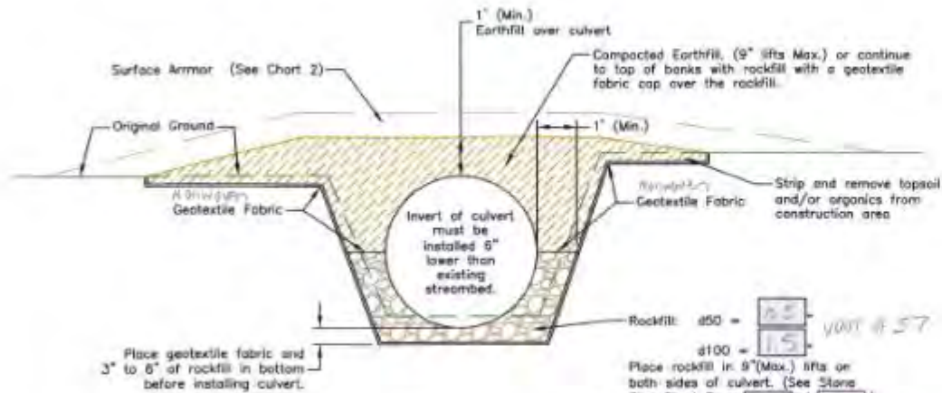
Single-Culvert Crossing Section Detail Not to Scale
