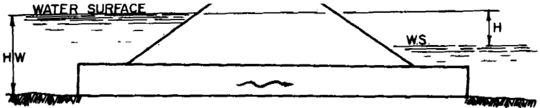
Figure 3-8 Culverts with outlet control
