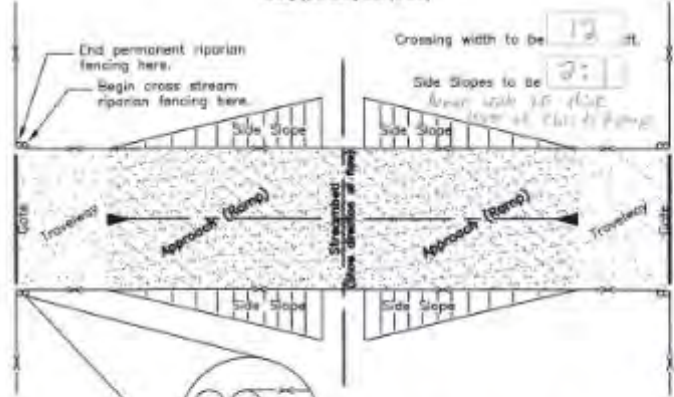
Typical Plan View (Showing riparian fencing and (in case))
