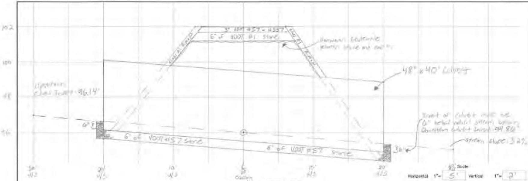
Stream Profile (On centerline of stream)
