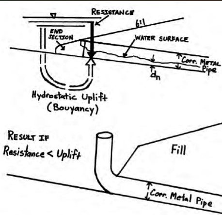
Figure 8-12. Hydrostatic Uplift Forces and Effects on Pipe
