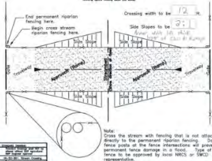
Typical Plan View Showing typical fencing detail (See notes)
