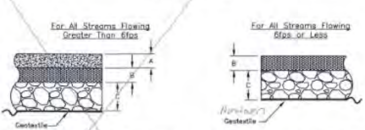
Typical Stone Layer
