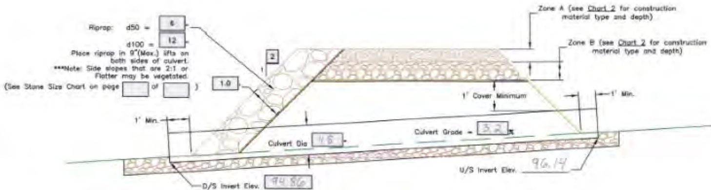
Culvert Crossing Profile Detail Not to Scale
