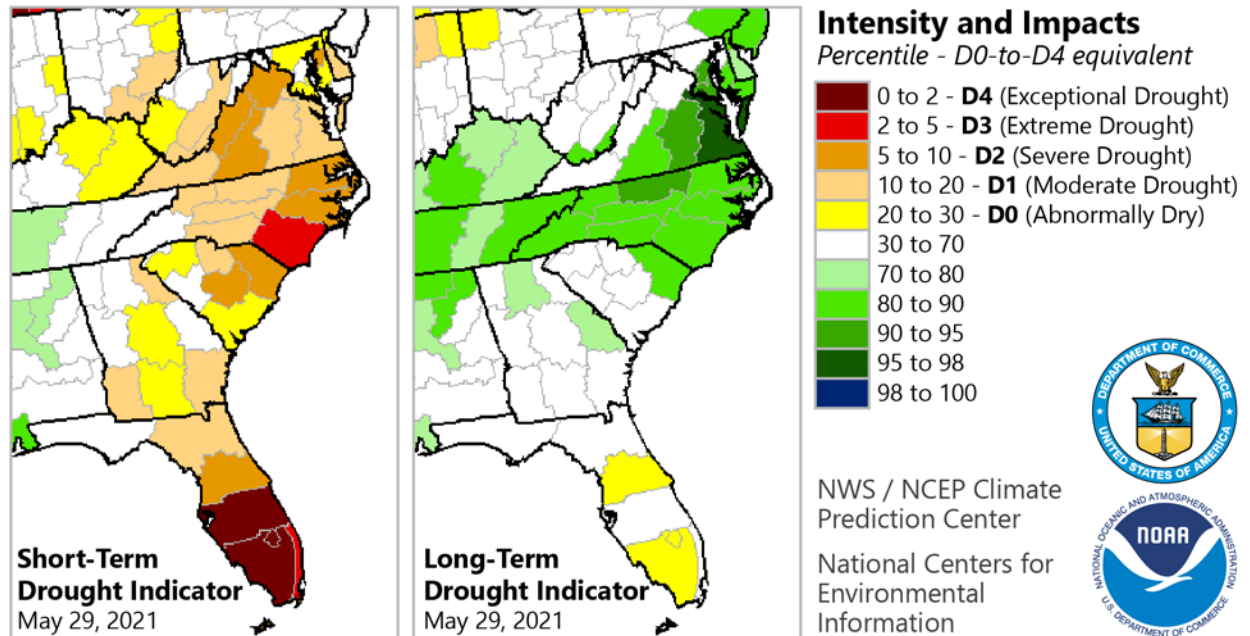
Figure 21: Examples of Short-Term and Long-Term Drought Prediction Maps, May 29, 2021 63
