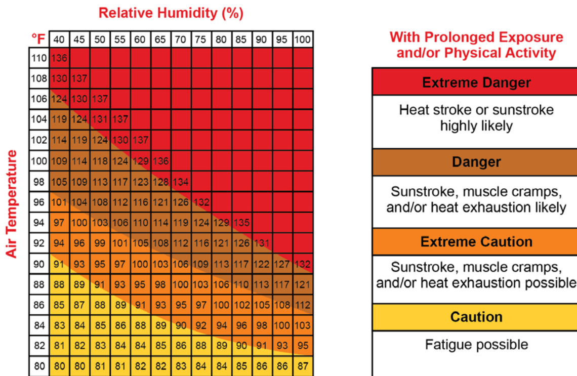
Figure 31: Heat Index and Relative Humidity, Effects on People 97
