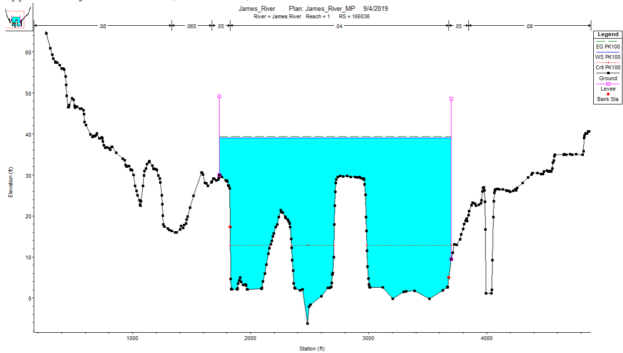
Figure 3: Model Cross Section at Mayo Island Bridge (14 th Street) From Preliminary Data
