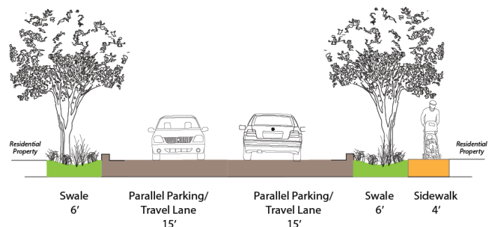
Example of how a sidewalk and stormwater swales can be incorporated within a portion of the right-of-way.
