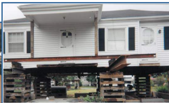
Photo II-2: Town of Glasgow, Flood Mitigation Project, 1997-2002
